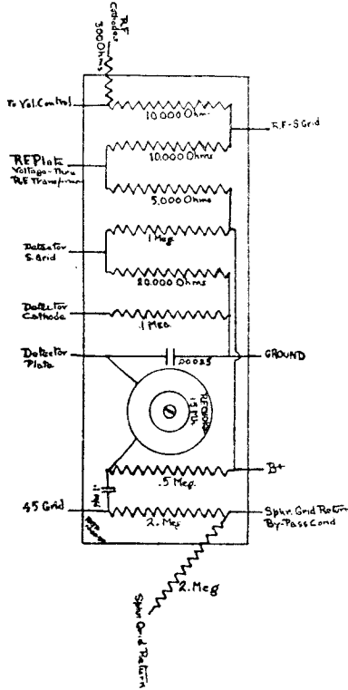
Resistor Strip
